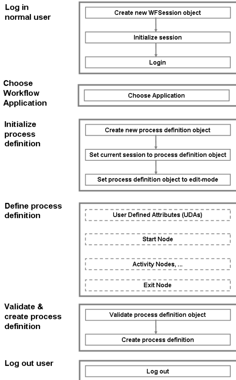
Figure 7: Designing a Process Definition Using the Model API
