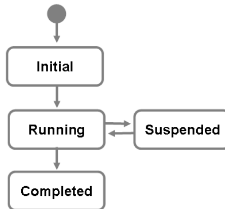
Figure 6: Process Instance State Transition Diagram
