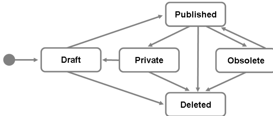
Figure 5: Process Definition State Transition Diagram
