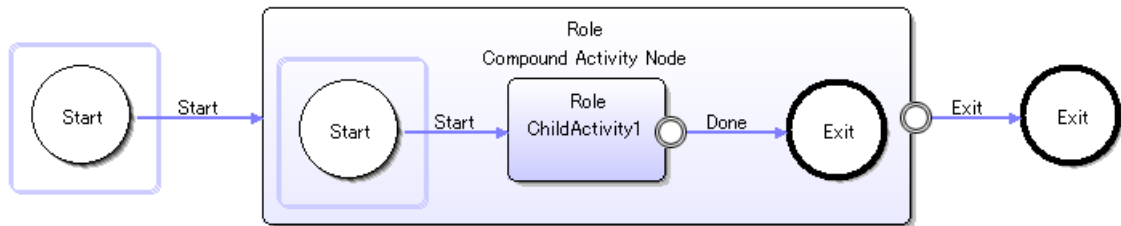
Figure 21: Compound Activity Node
