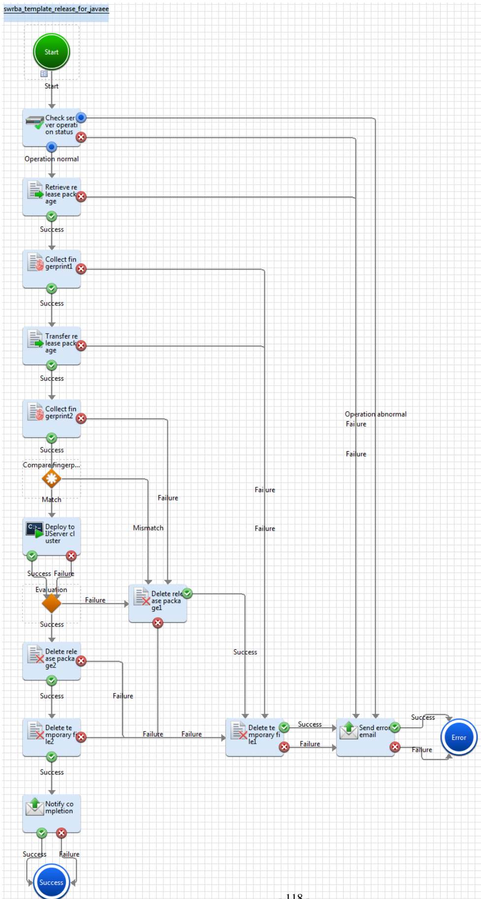
Figure 7.9 Release automation template example
