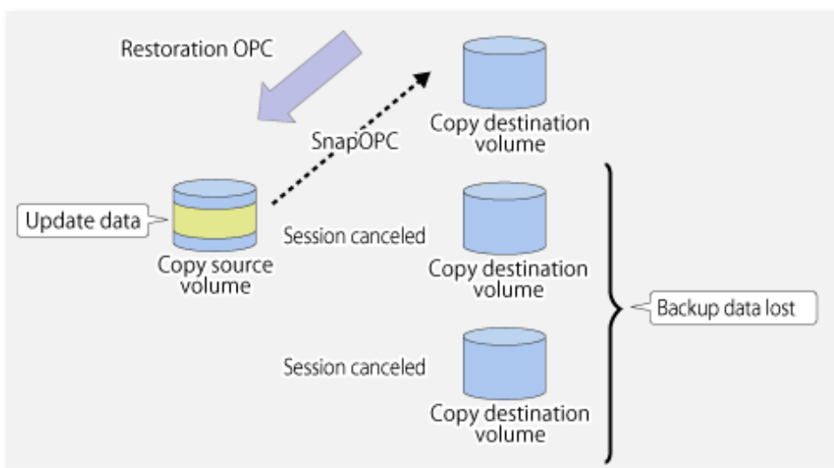
Figure 6.26 When SnapOPC session cancelled to perform restoration
