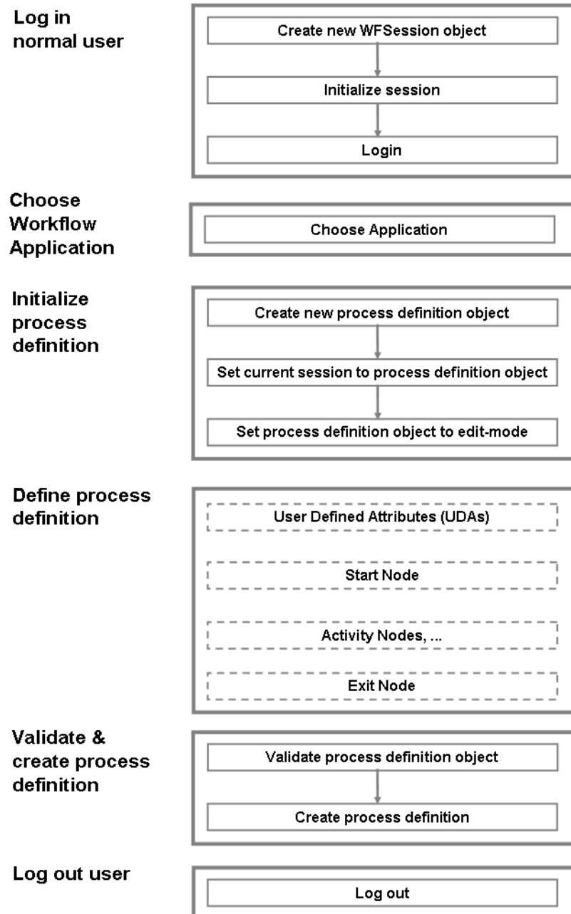
Figure 6: Designing a Process Definition Using the Model API
