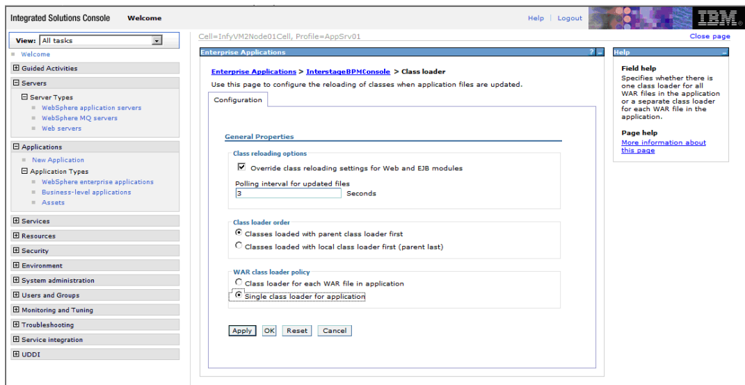
Figure 22: Enterprise Application Class Loader Details Page
