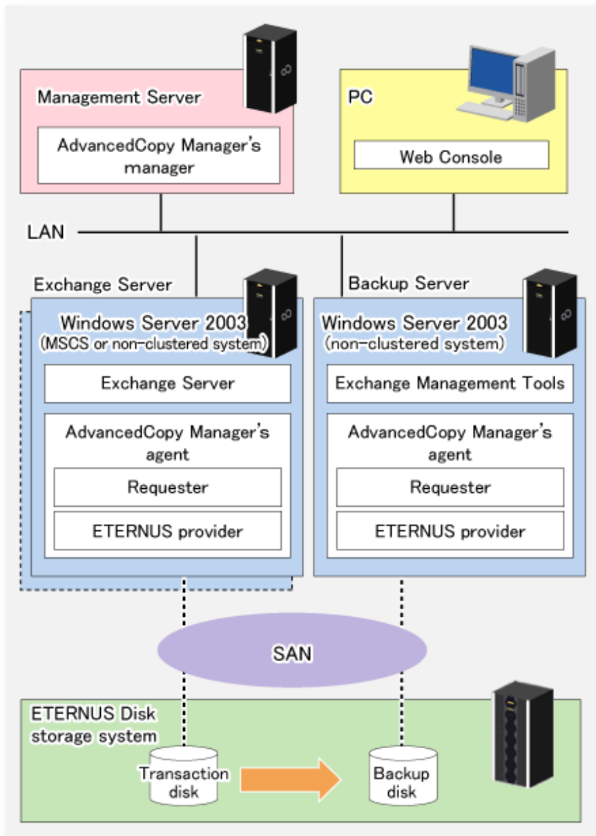
Figure 7.5 System configuration
