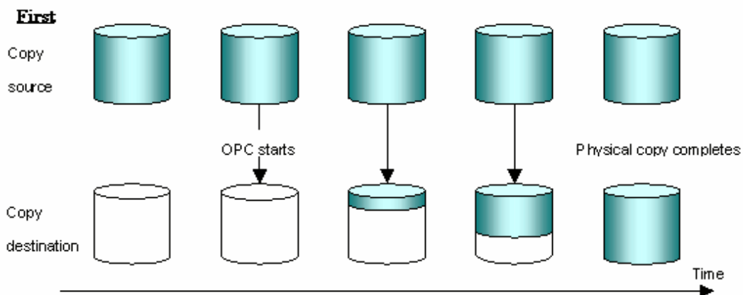
Figure 8.3 QuickOPC replication
