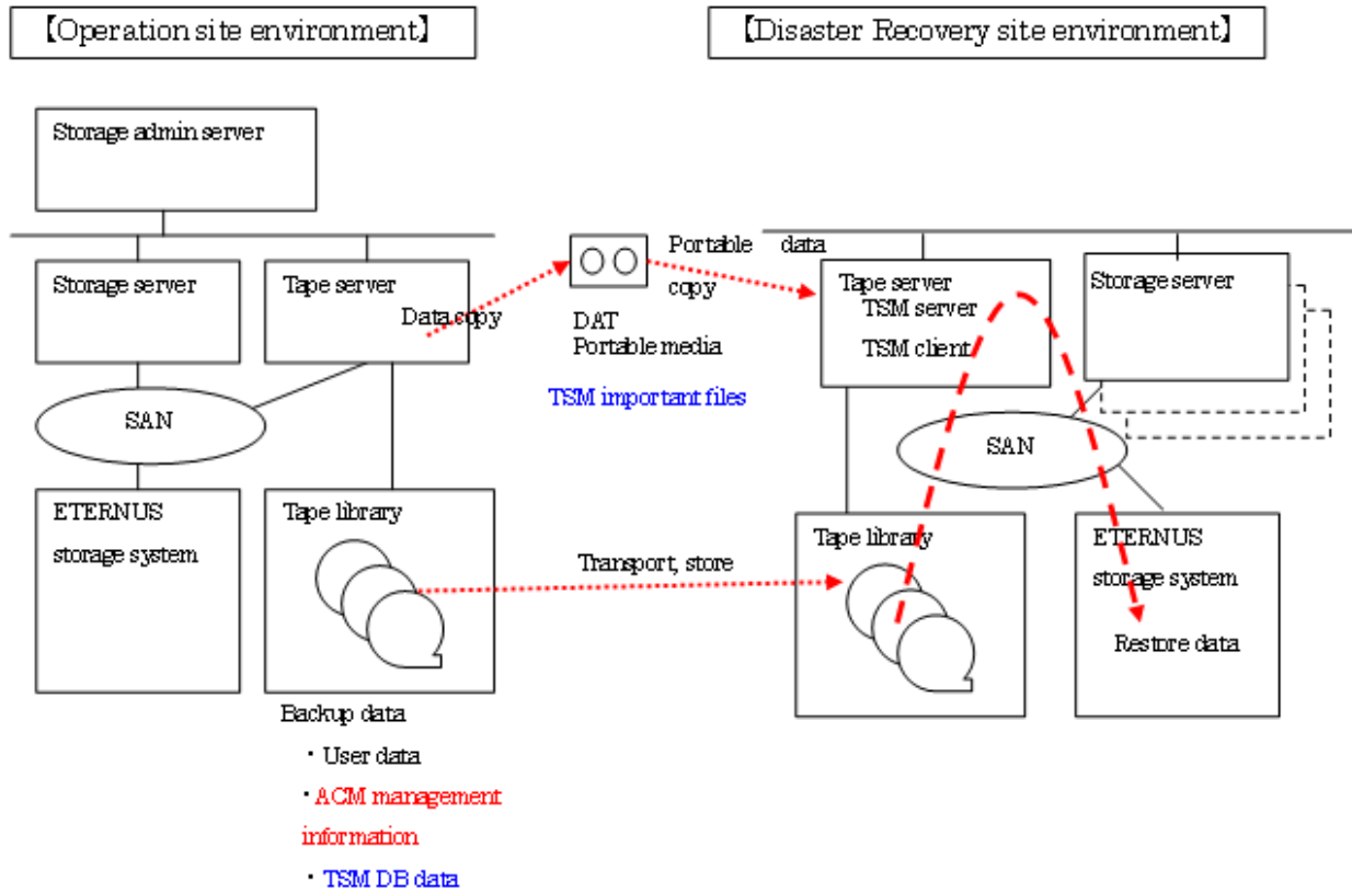
Figure 14.1 Flow of data restoration at the operation site and the disaster recovery site
