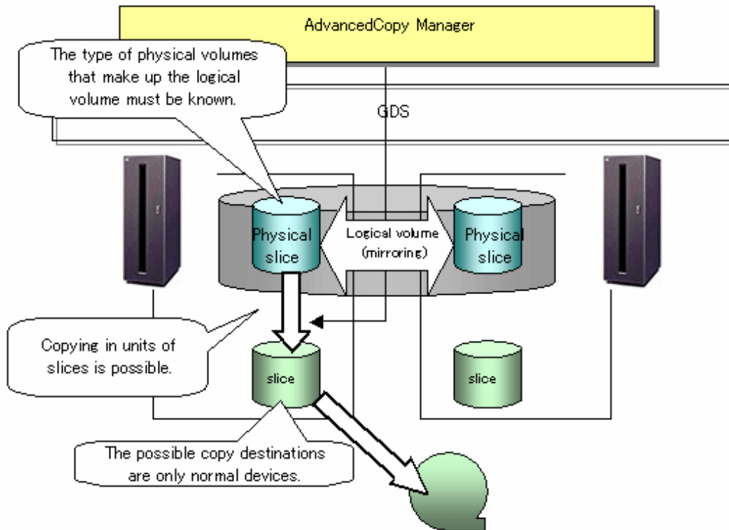
Figure 5.15 Backup operation in units of slices
