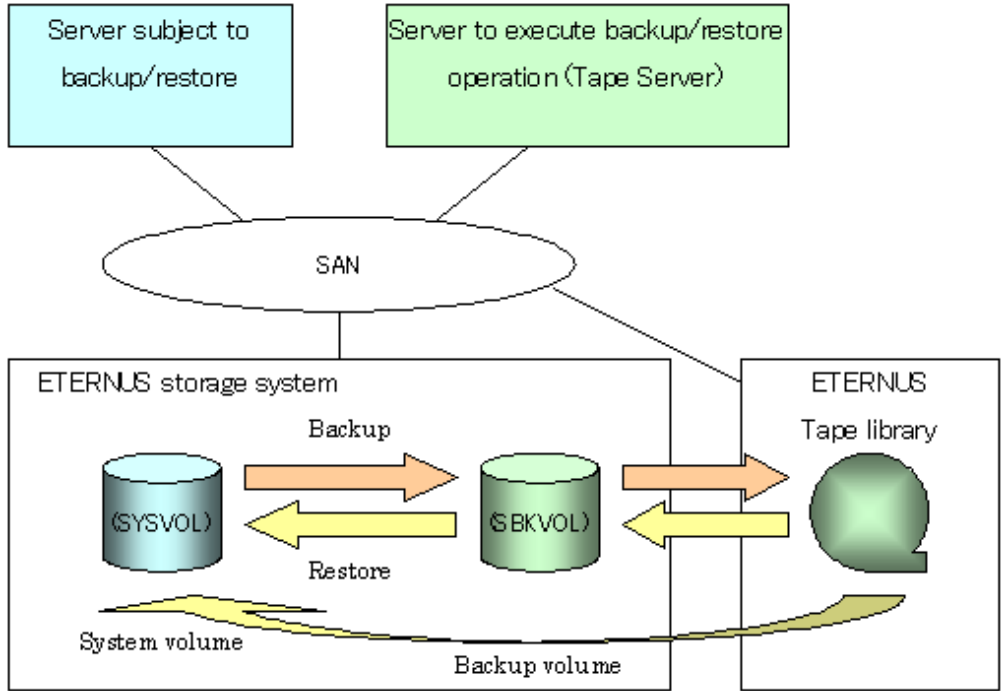
Figure C.3 Configuration example when a backup volume is used to backup to tape media
