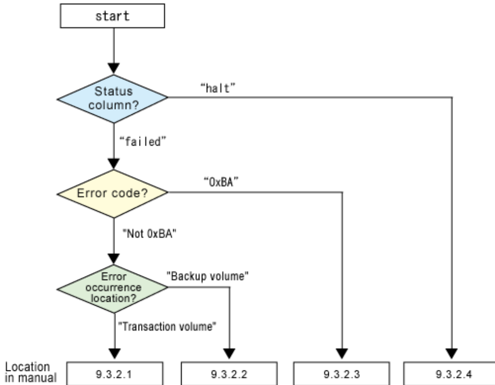
Figure 9.1 Troubleshooting flow when hardware errors occur
