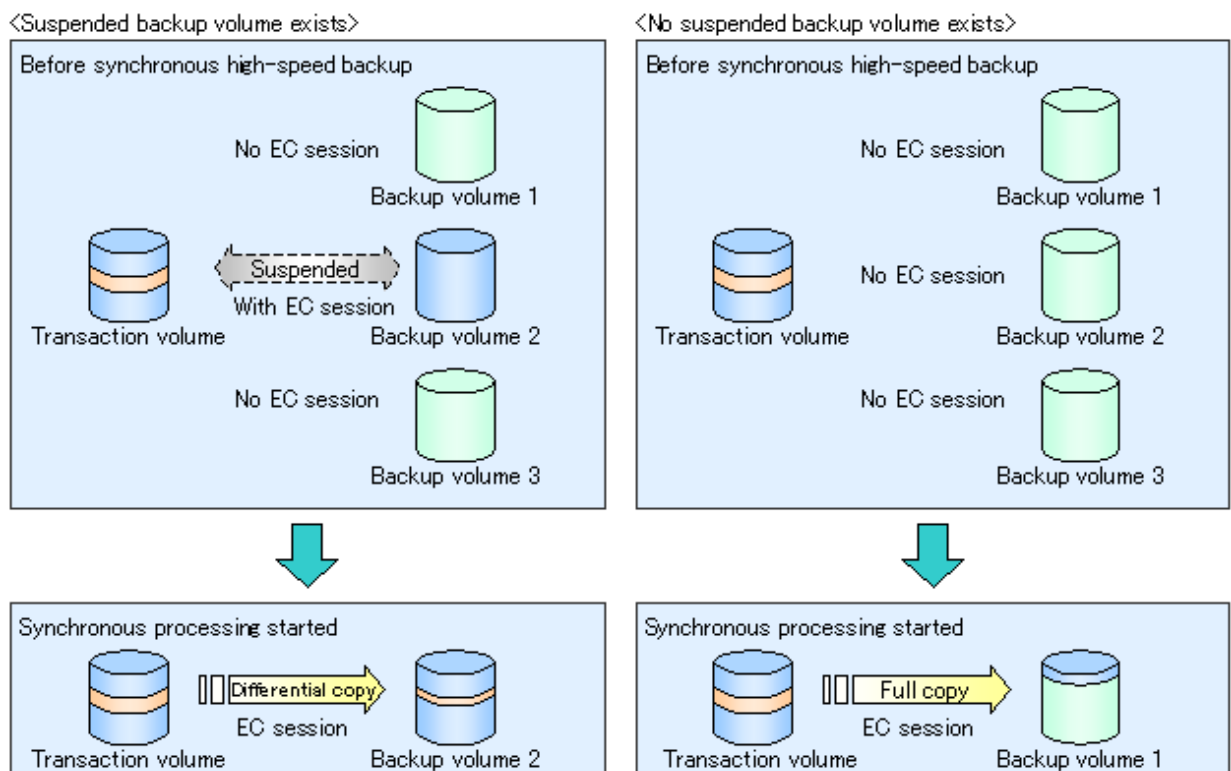
Figure 5.10 Backup volume selection at start of synchronous processing
