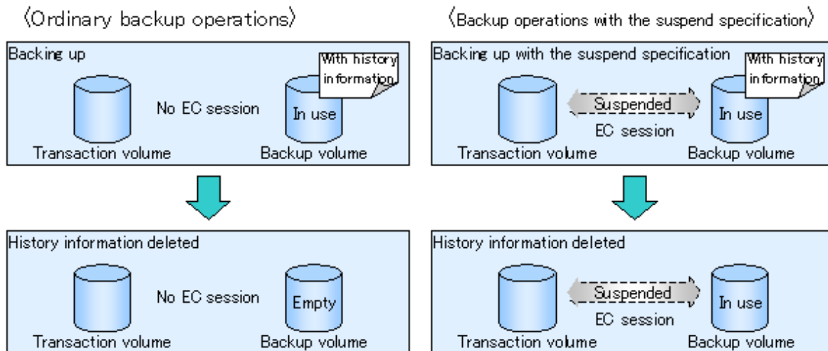
Figure 5.14 Deletion of an ordinary backup history and the deletion of backup history with the suspend specification
