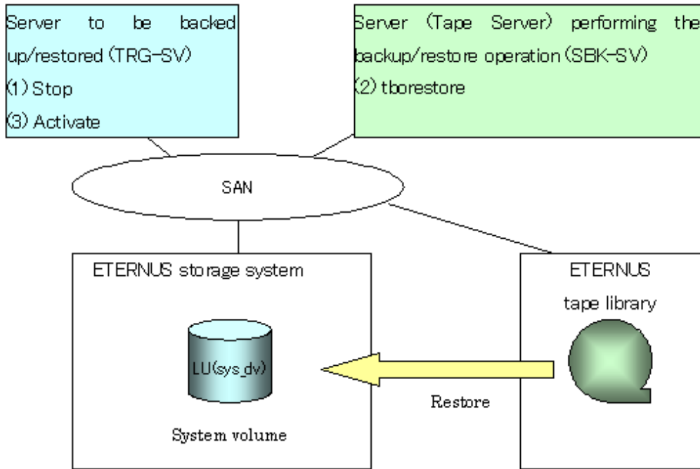
Figure C.12 Restoring from tape
