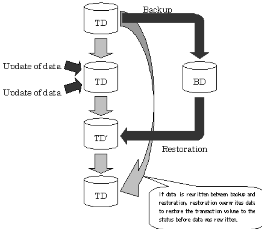
Figure 5.8 Notes on restoration with AdvancedCopy Manager
