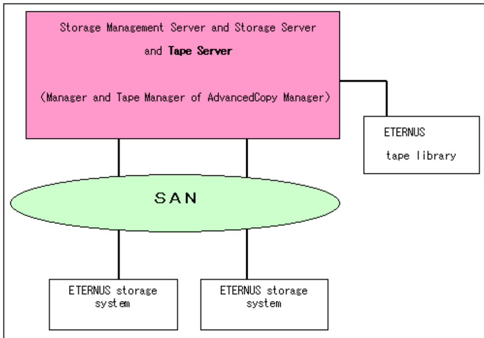
Figure 1.2 When the Tape Server is also operated as the Storage Management Server
