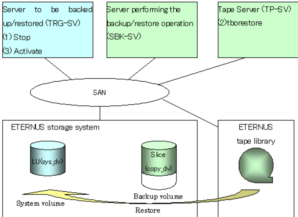
Figure C.11 Restoring from tape to system volume (LU)
