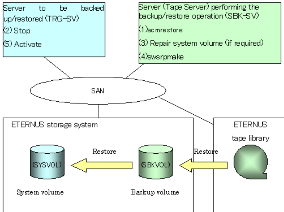
Figure C.10 Restoring from tape using a backup volume
