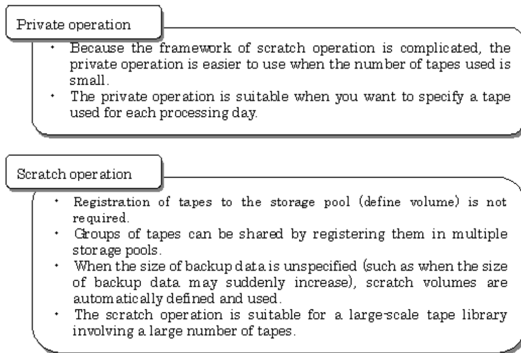
Figure 3.1 Private operation and scratch operation selection criteria
