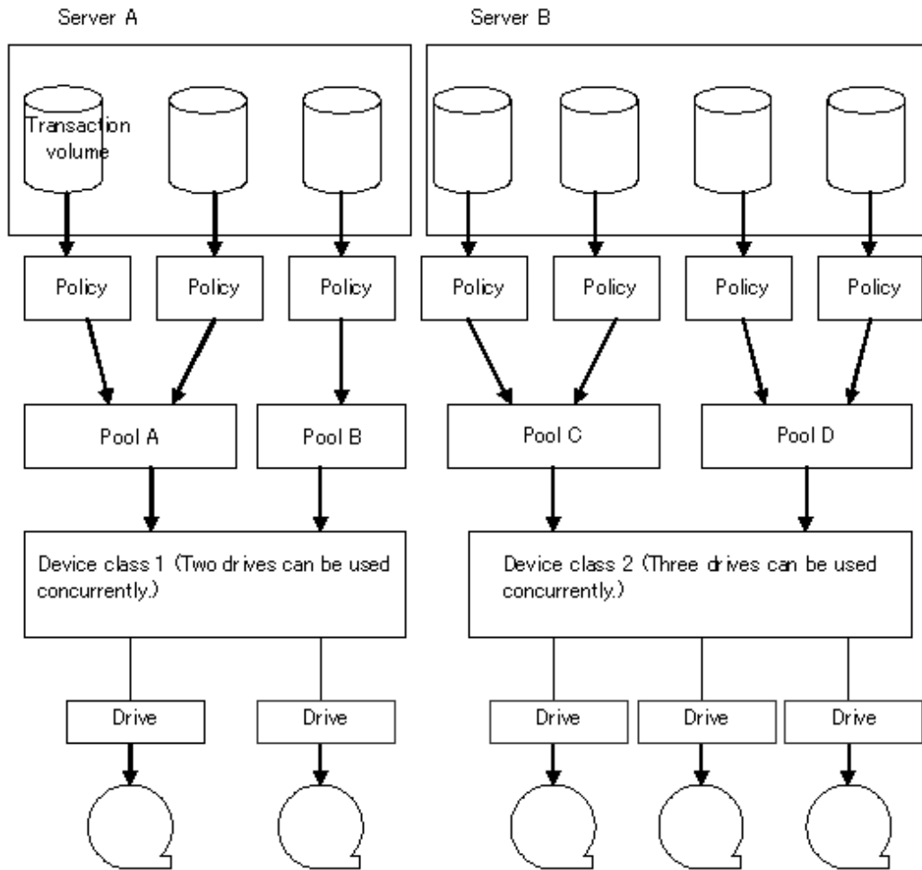
Figure 3.3 Relationships between transaction volumes and definitions
