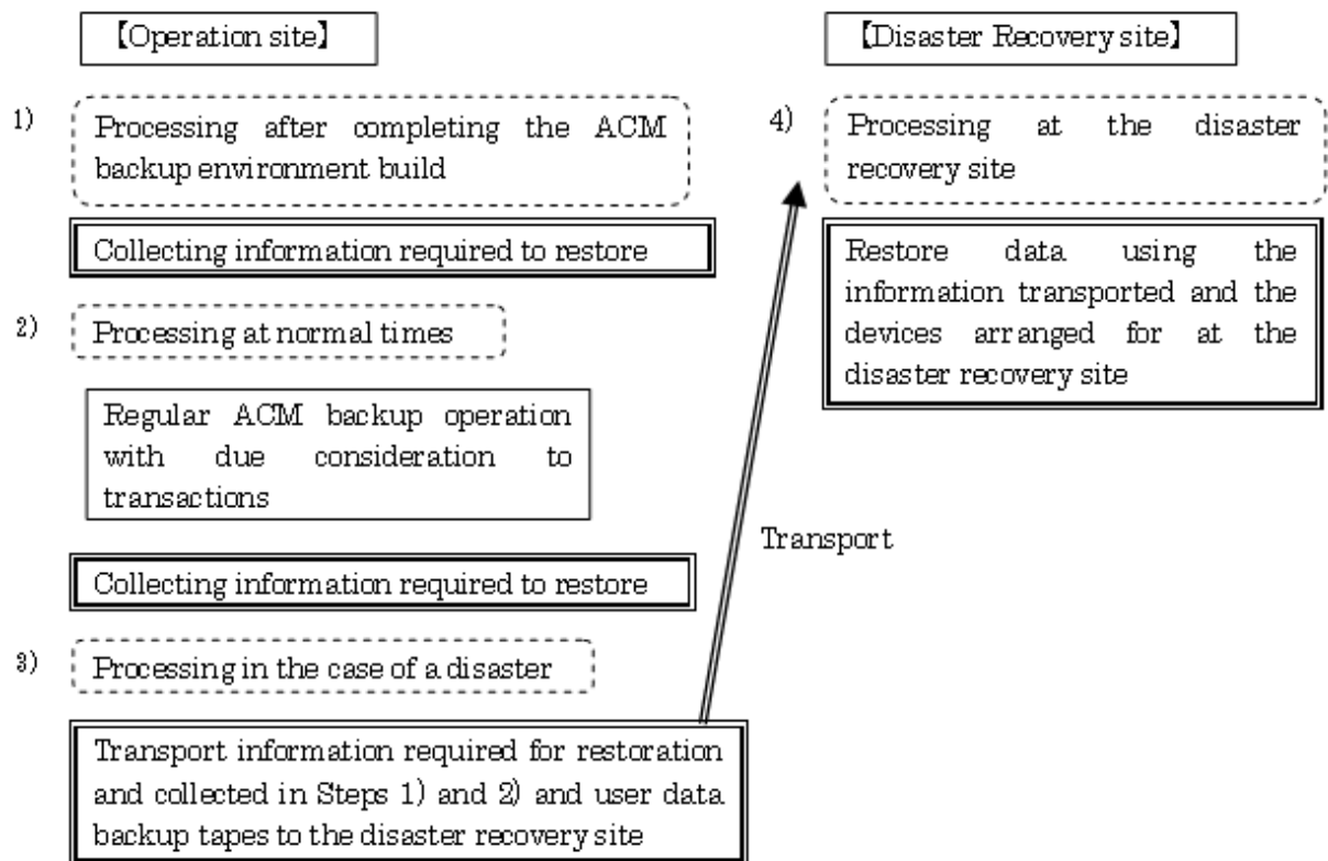
Figure 14.3 Data restoration flow
