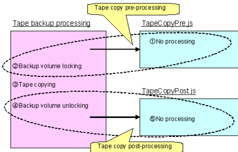
Figure A.1 Relationship between backup volume locking/unlocking and pre-processing and post-processing of the script
