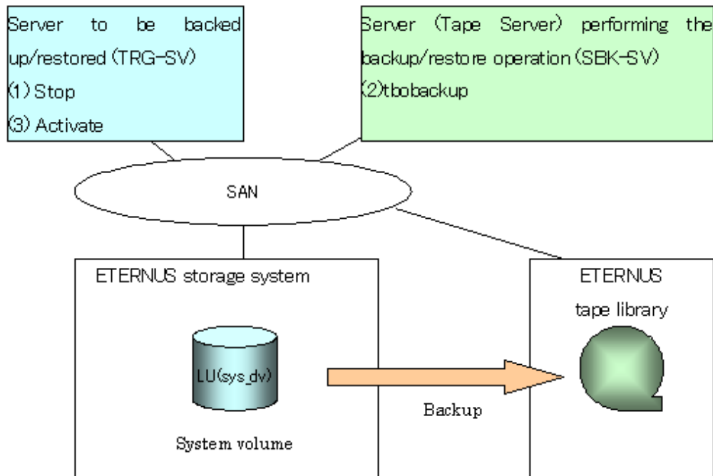
Figure C.8 Backing up directly to tape
