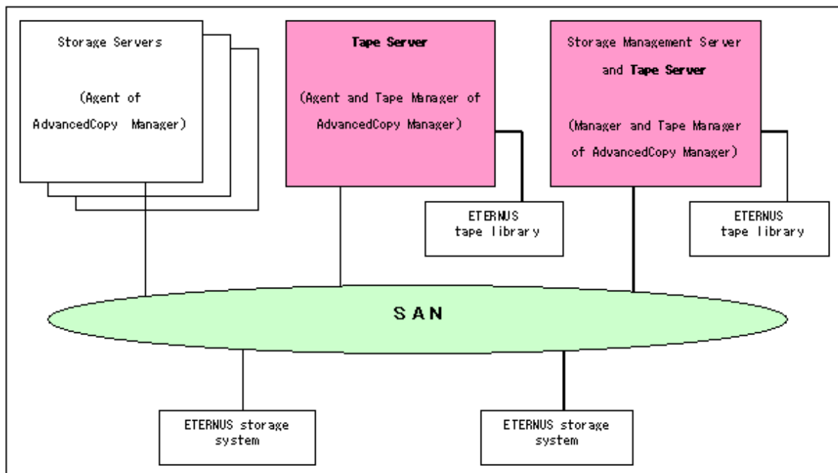
Figure 1.5 When an ETERNUS tape library is not shared
