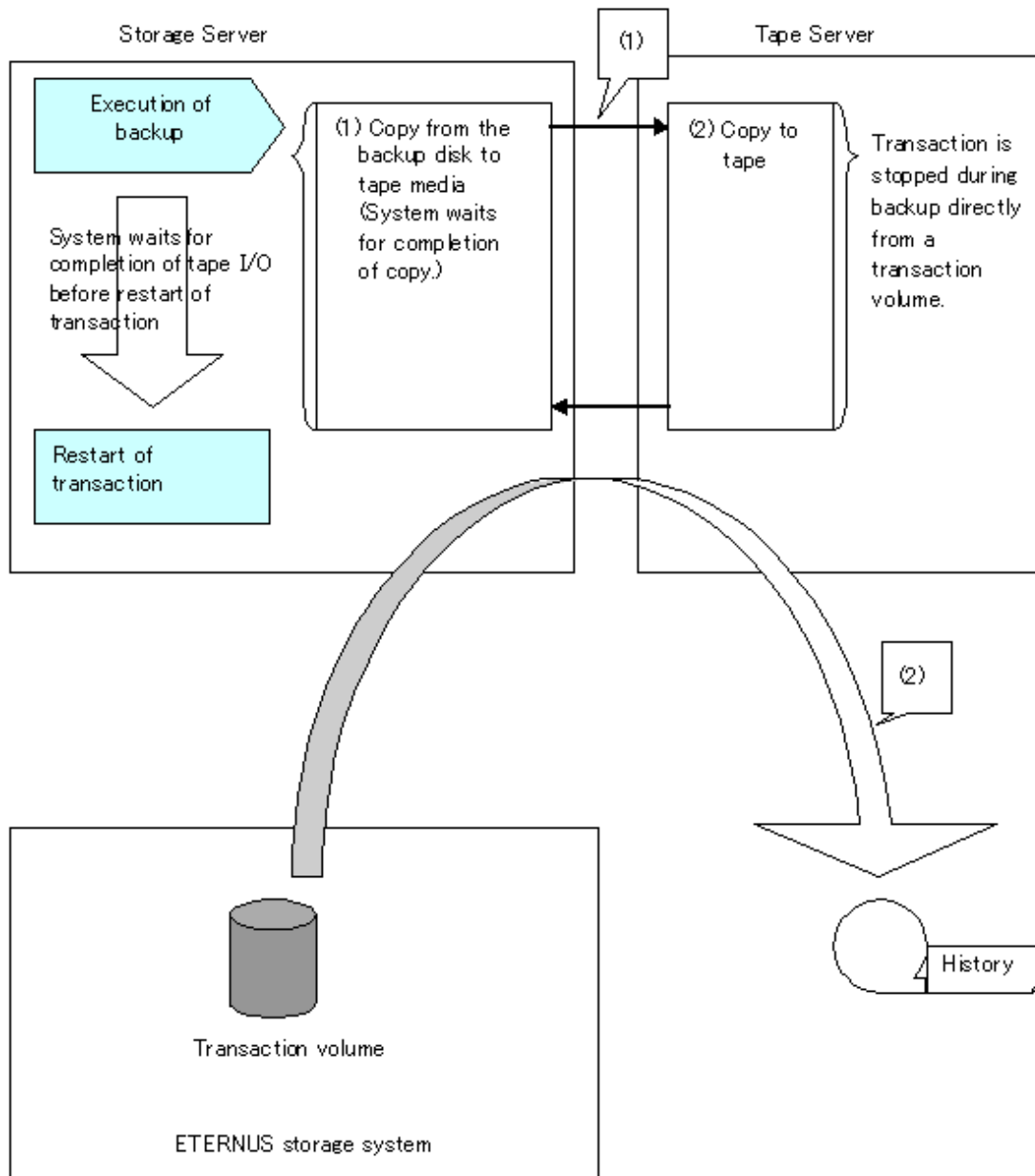
Figure 1.8 Method for direct backup to tape
