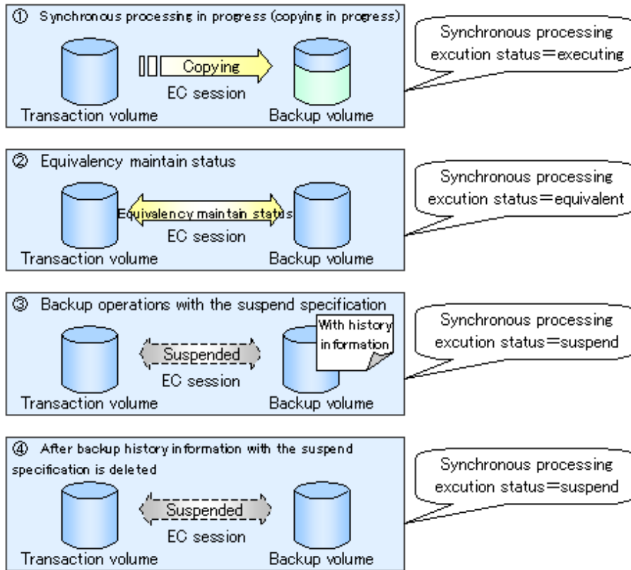
Figure 5.11 Progress information displayed by the synchronous processing progress display command
