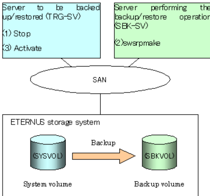
Figure C.6 Backing up to a backup volume
