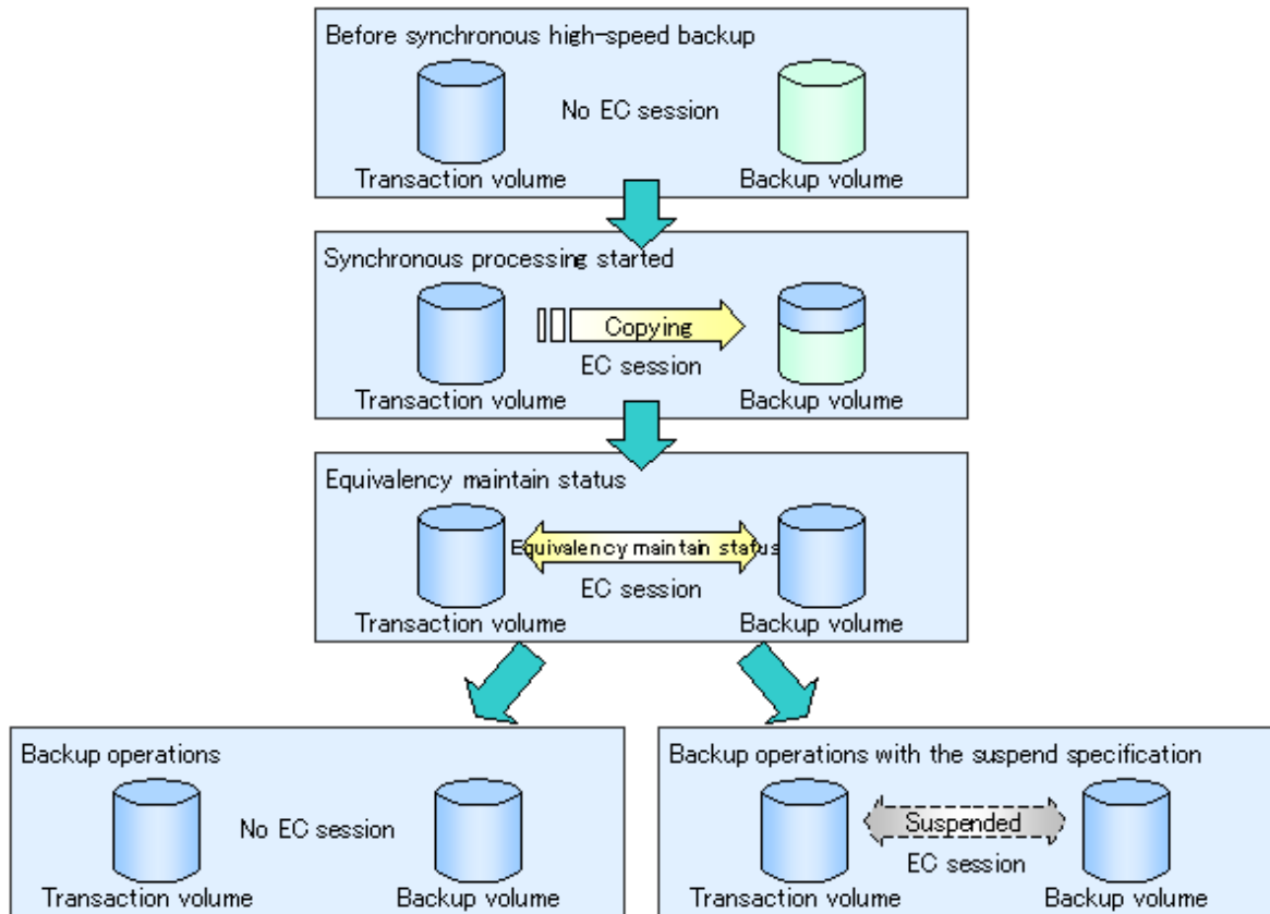
Figure 5.12 Ordinary backup, and backup with the suspend specification
