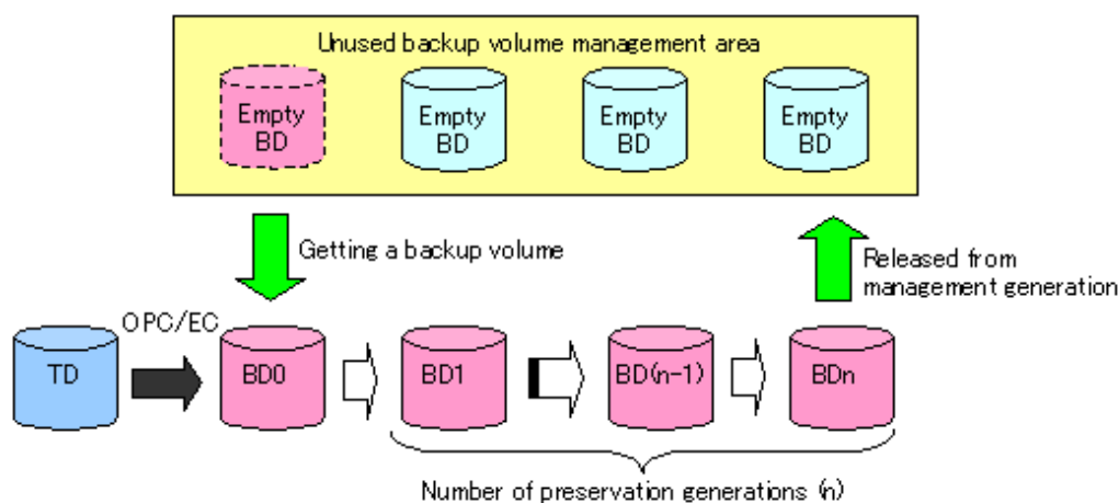
Figure 5.1 Backup volume management
