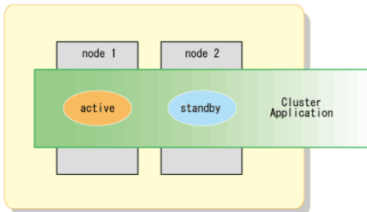
Figure 1.1 1:1 standby system
