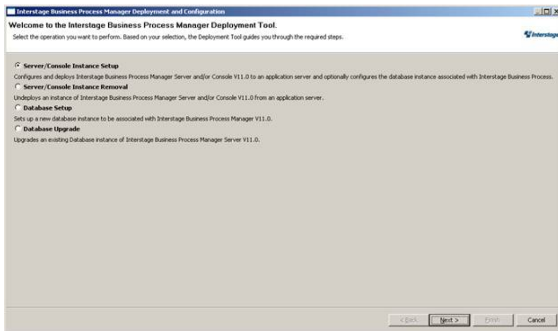
Figure 10: Welcome
