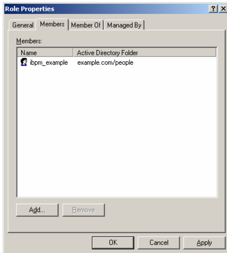
Figure 33: Adding Members
