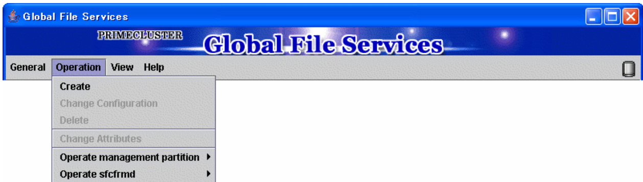
Figure 7.5 Operation menu
