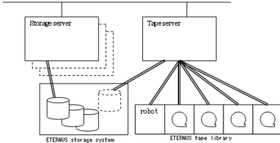
Figure 14.2 Hardware diagram of the disaster recovery site
