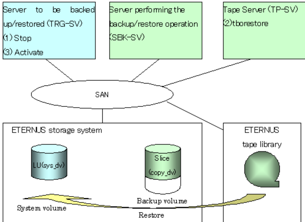
Figure C.11 Restoring from tape to system volume (LU)
