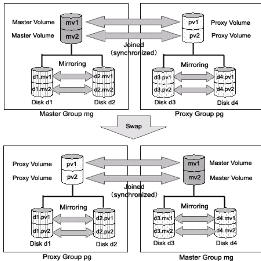
Figure: Swapping Master Group and Proxy Group
