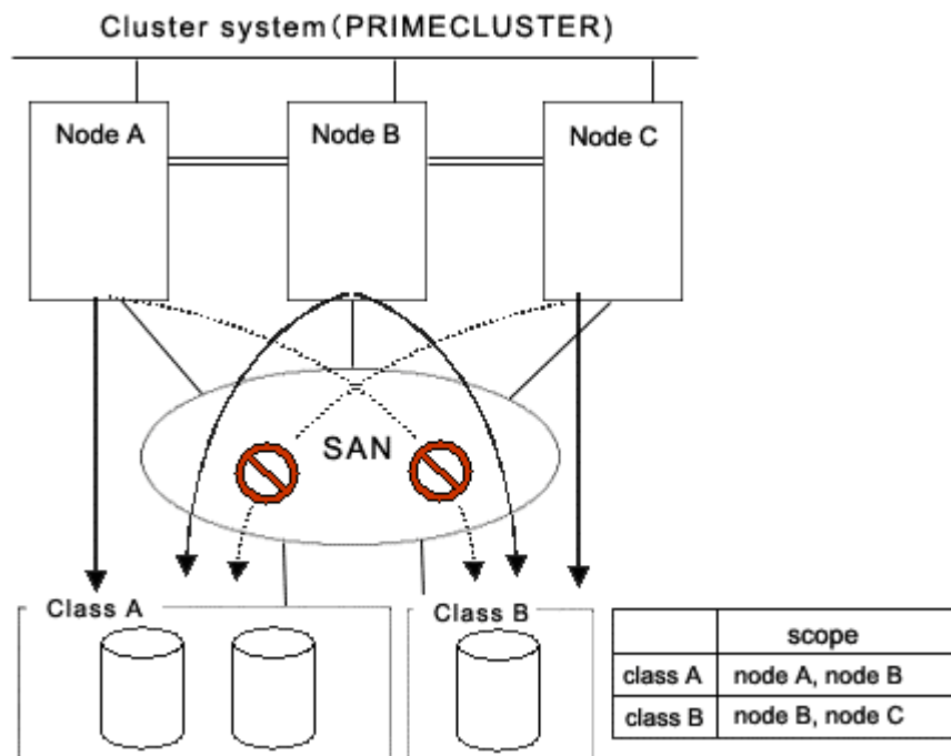
Figure: Class Scope
