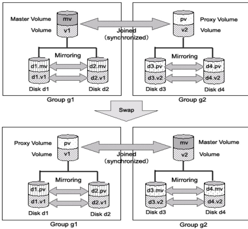
Figure: Swapping Master Group and Proxy Group
