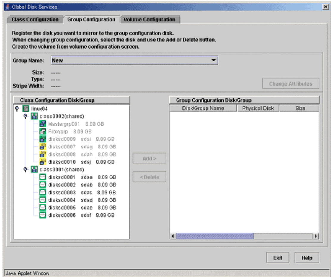
Figure: Group Configuration
