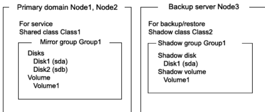
Figure: Object Configuration When Backing Up
