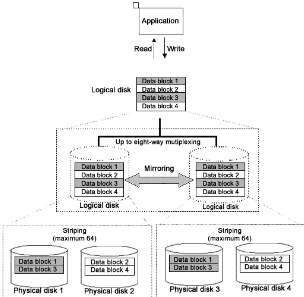
Figure: Combining Striping and Mirroring
