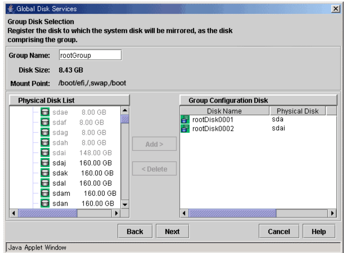
Figure: Group Disk Selection: rootGroup
