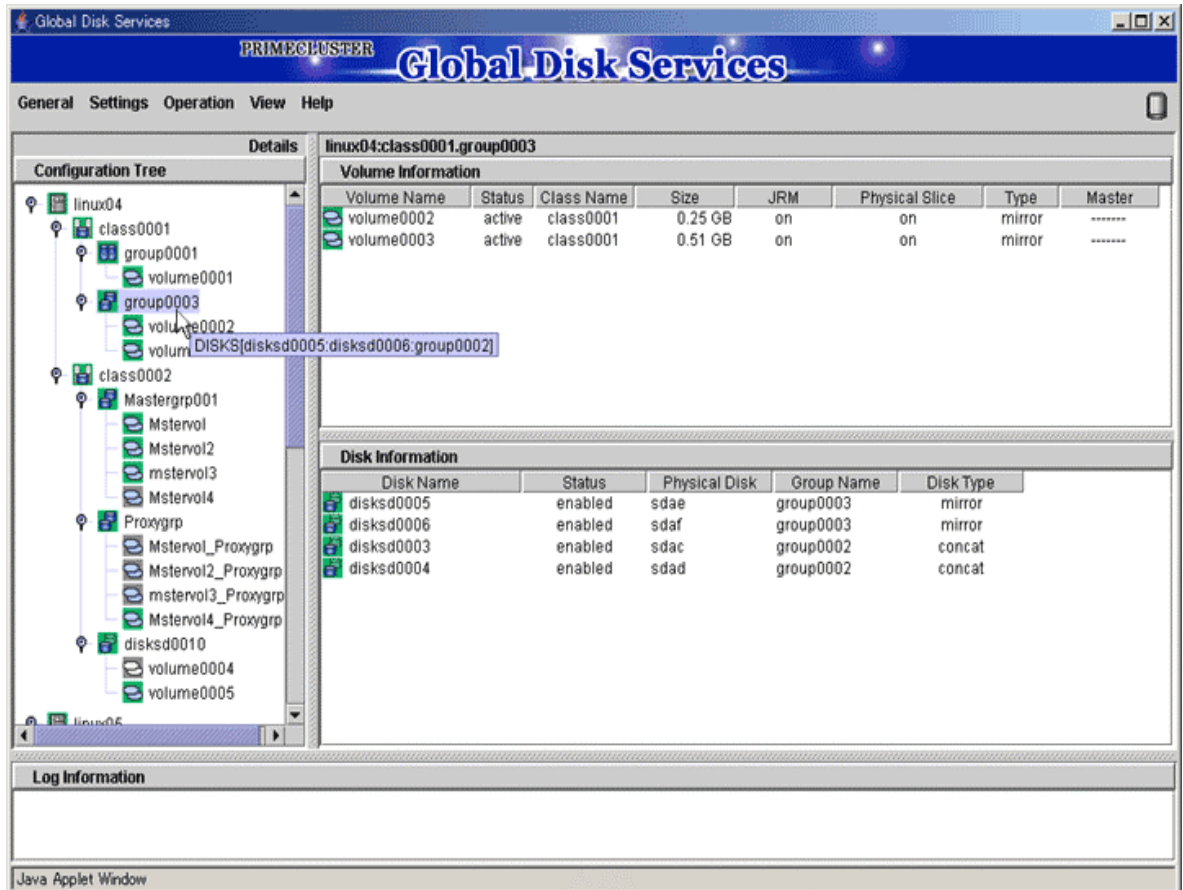
Figure: Main Screen (for SDX Objects of a Group)
