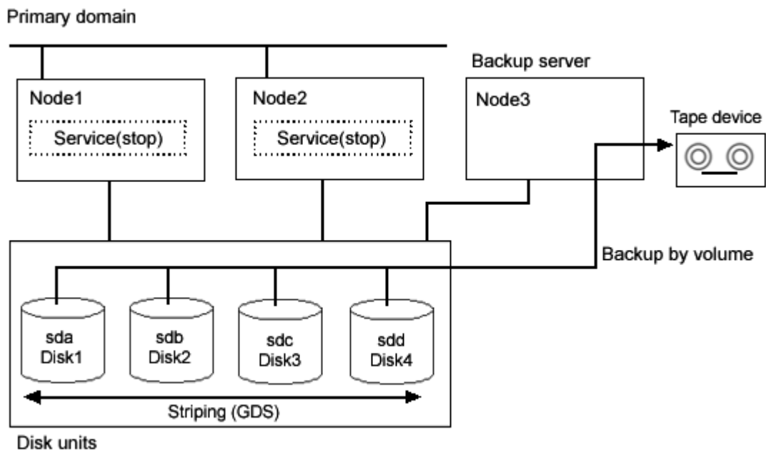
Figure: Object Configuration When Backing Up
