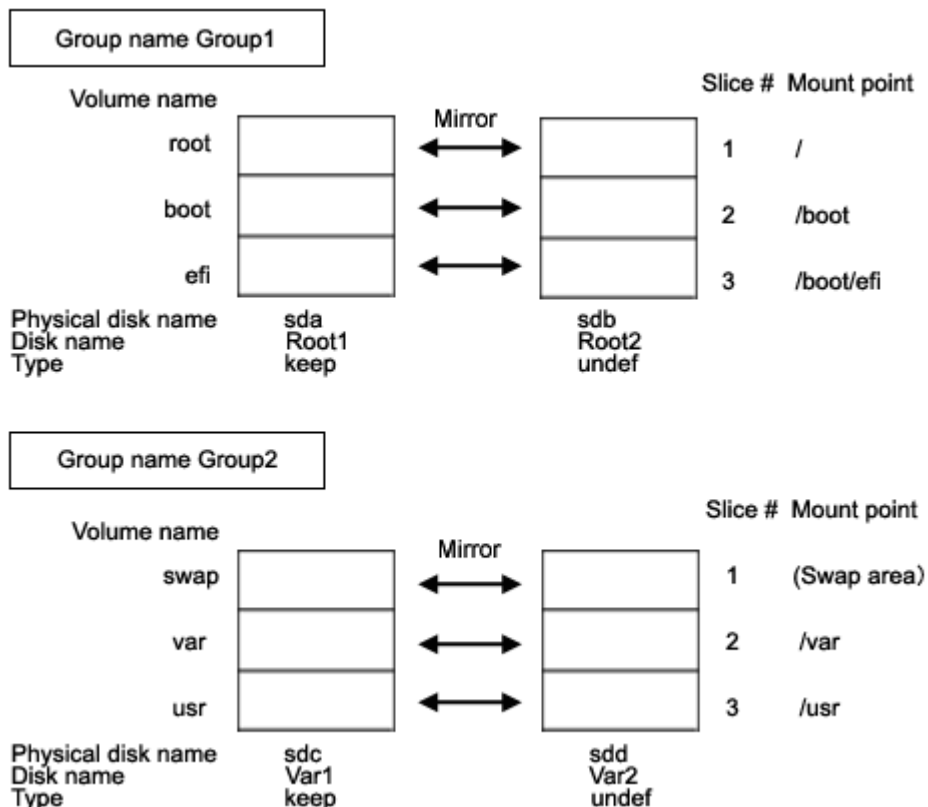
Figure: System Disk Configuration
