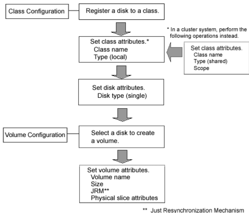
Figure: Single Volume Configuration Settings Operation
