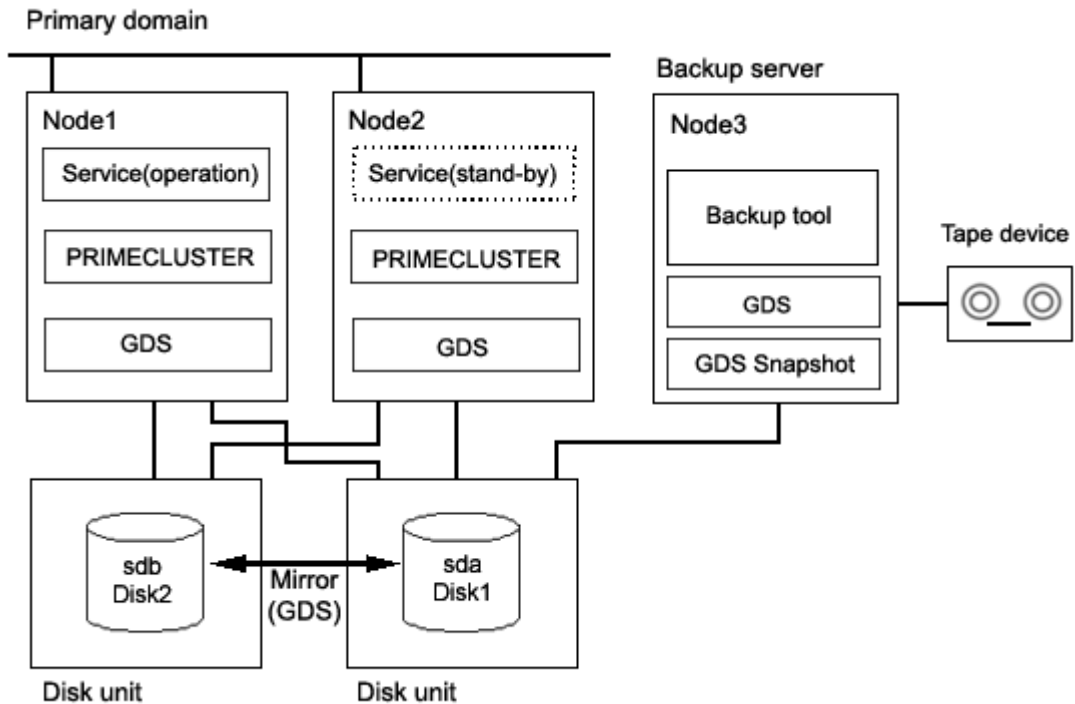
Figure: System Configuration
