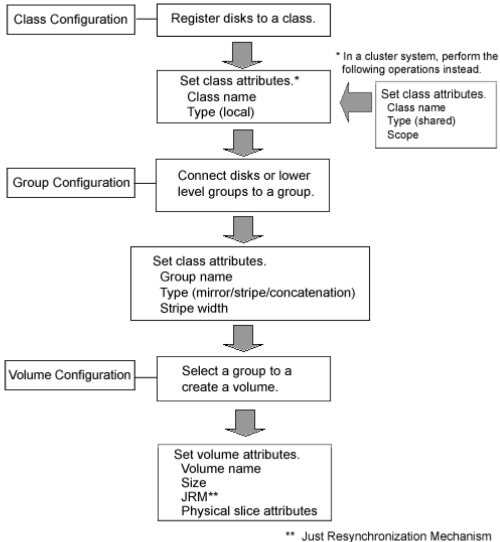
Figure: Volume Configuration Settings Operation
