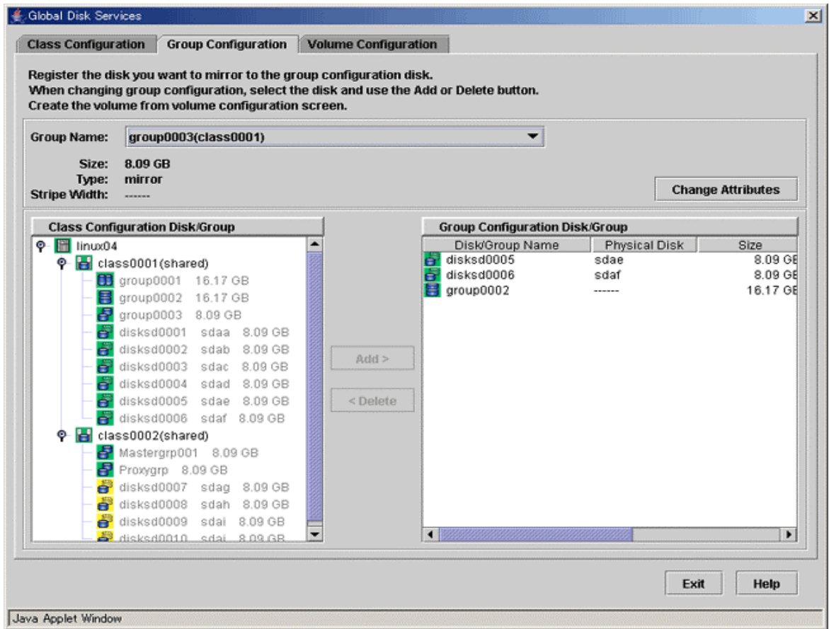
Figure: Confirming Group Configuration Group/Disk
