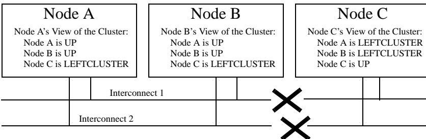
Figure 57: Three-node cluster where connection is lost
