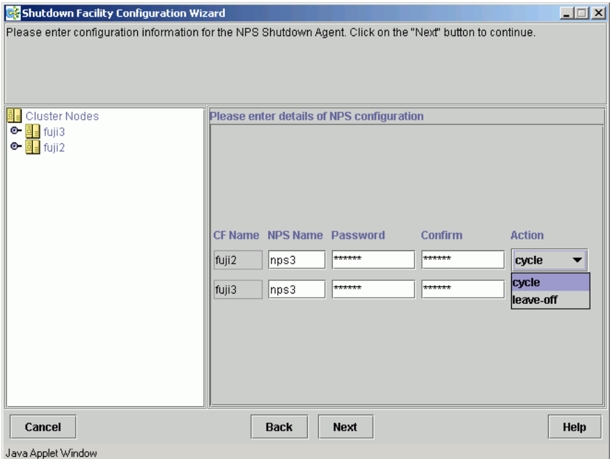
Figure 68: Configuring the NPS Shutdown Agent
