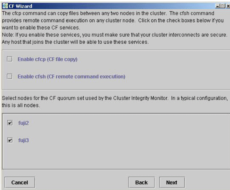
Figure 16: CIM configuration window
