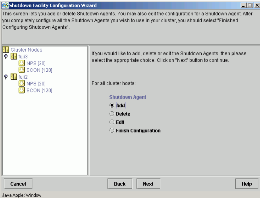
Figure 73: Adding, deleting, editing Shutdown Agents
