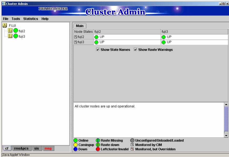
Figure 21: Main CF window
