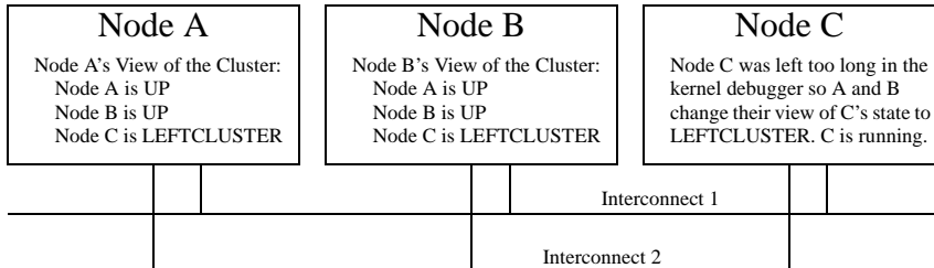
Figure 58: Node C placed in the kernel debugger too long
