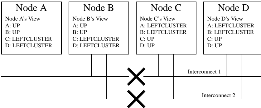
Figure 59: Four-node cluster with cluster partition
