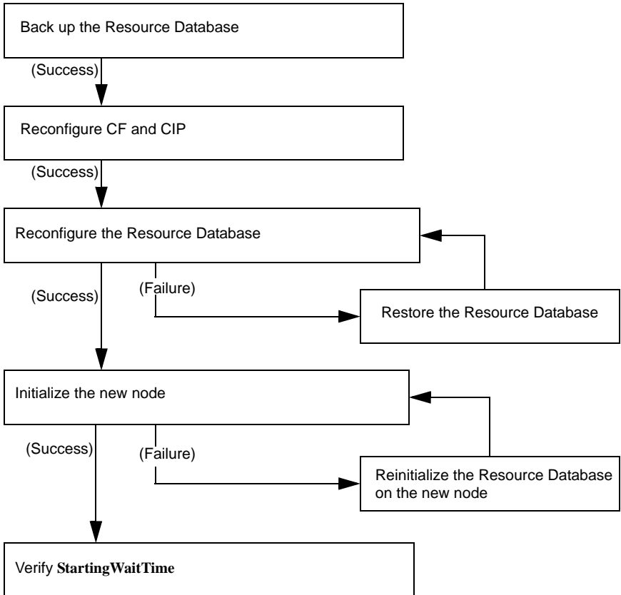
Figure 22: Adding a new node
