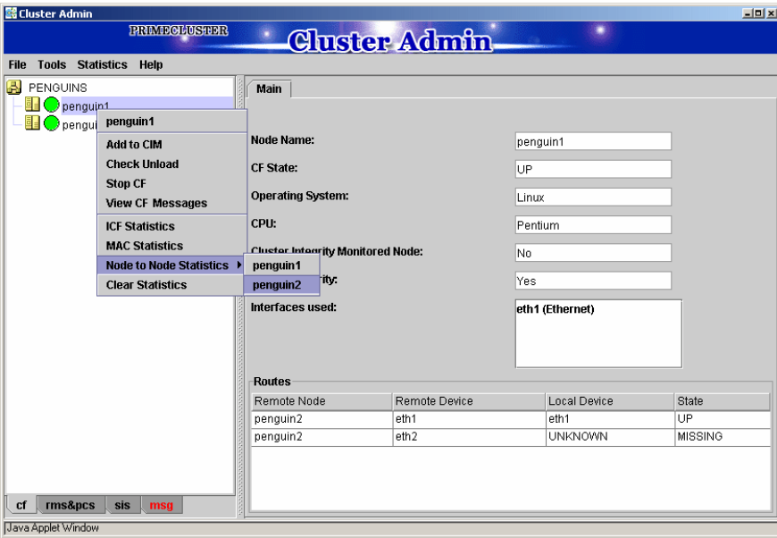
Figure 46: Selecting a node for node to node statistics
