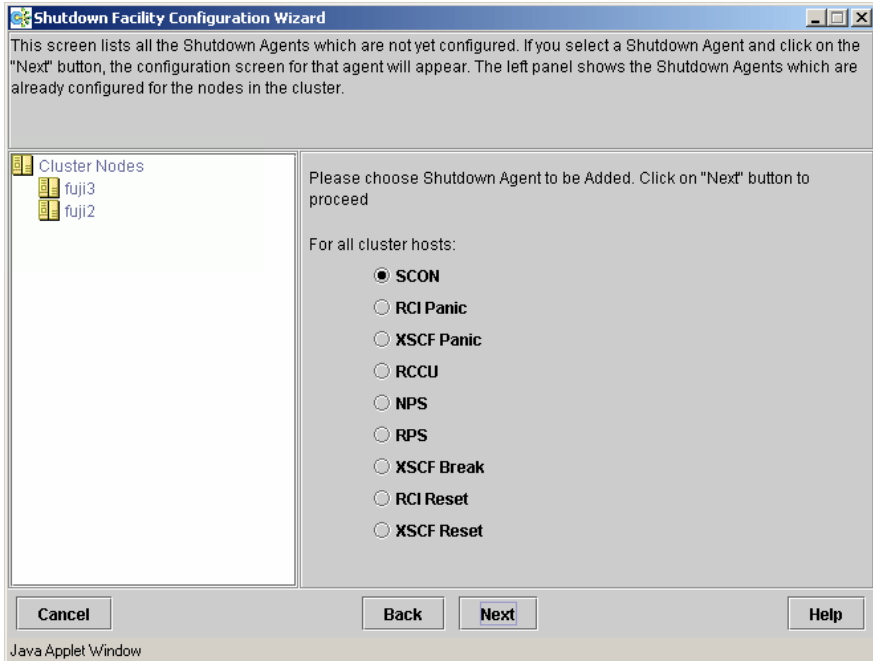
Figure 67: Choose Shutdown Agent to be added
