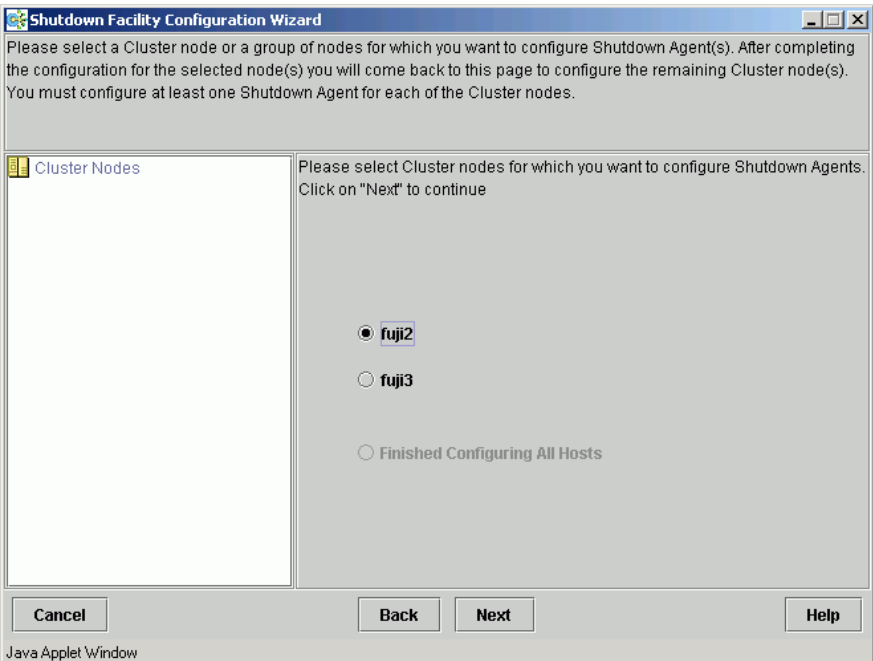
Figure 66: Selecting nodes to configure Shutdown Agents
