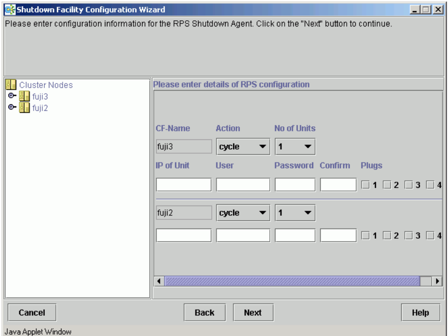
Figure 70: Configuring the RPS Shutdown Agent
