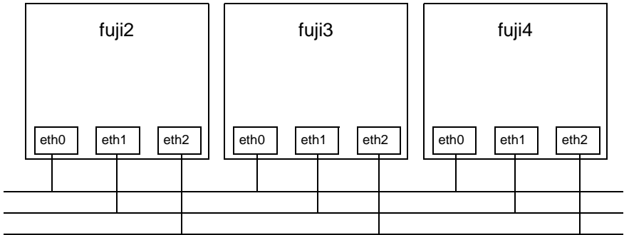
Figure 60: A three-node cluster with three full interconnects
