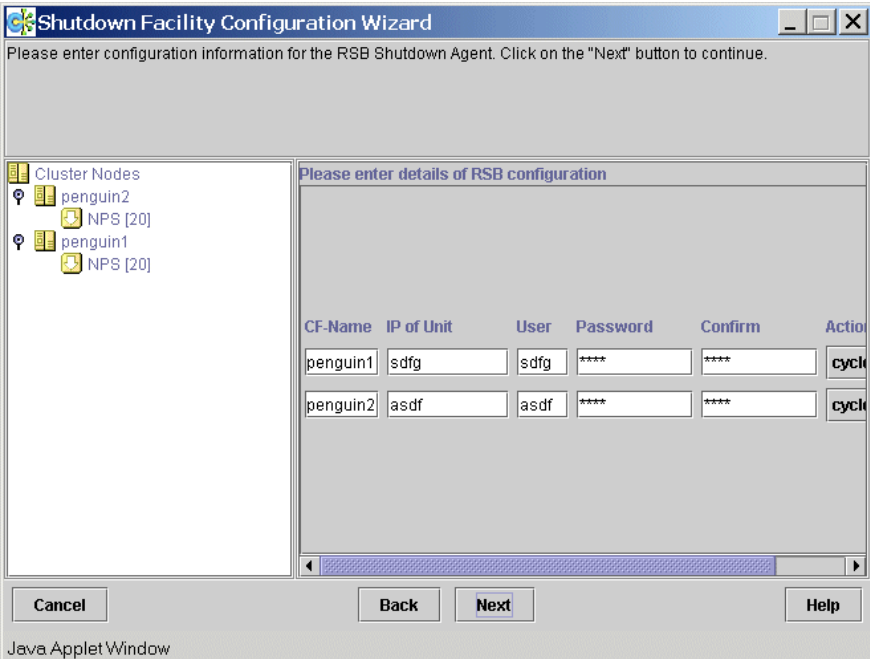
Figure 69: Configuring the RSB Shutdown Agent
