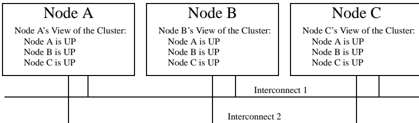
Figure 56: Three-node cluster with working connections
