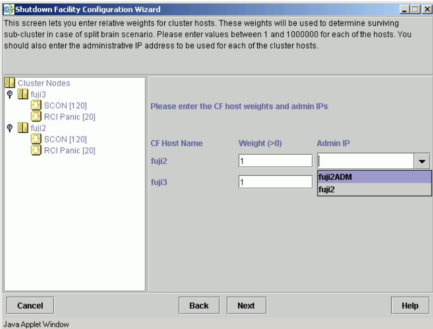
Figure 77: Entering node weights and administrative IP addresses
