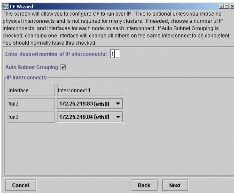
Figure 14: CF over IP window
