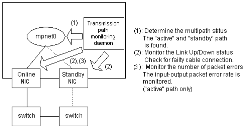
Figure 2.3 Fault Monitoring of Multipath Function
