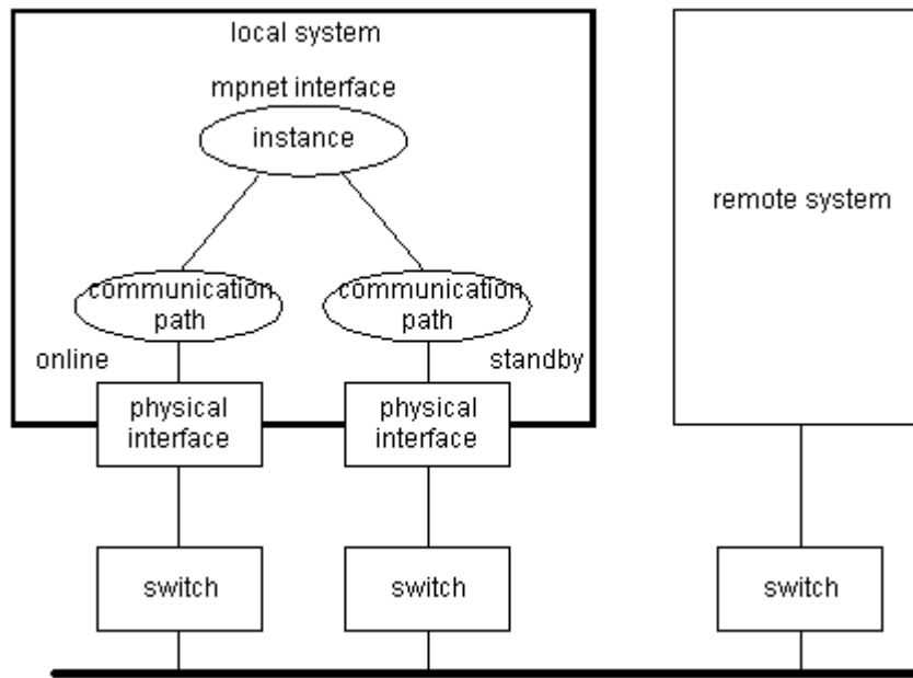
Figure 2.2 System Configuration of Multipath Function
