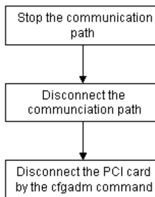
Figure 8.2 Disconnection Procedure
