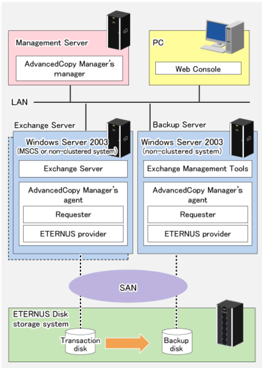
Figure 7.5 System configuration
